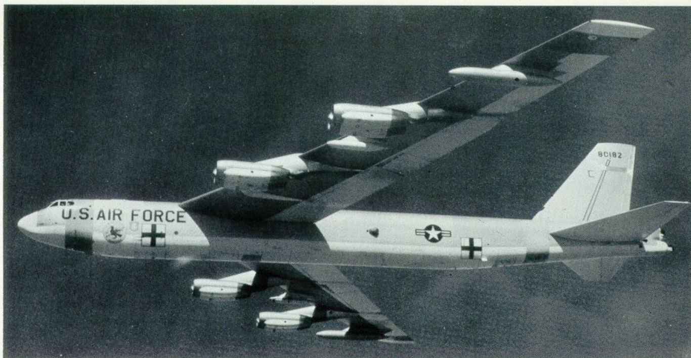
A B-52G with 700-gallon (U.S.) drop tanks being used by the Air Force to test electronic countermeasures pods that can be seen under the wings between the inboard and outboard nacelles. Note the double theodolite target markings fore and aft on the fuselage. (Photo: USAF via Boeing)
