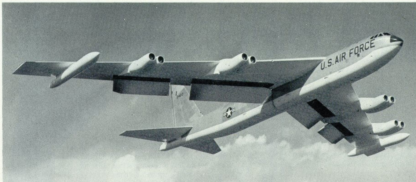
Flight view of a B-52C with flaps fully extended. Note that flaps are divided in the area immediately behind the inboard engines. Drop tanks are 3000-gallon (U.S.) capacity. (Photo: Boeing)
