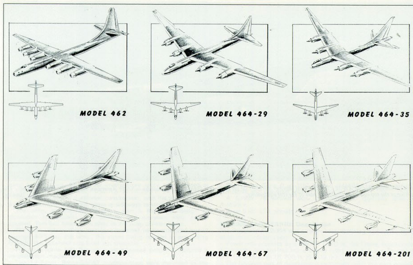
Six stages of developing the B-52 Stratofortress.
